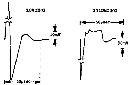
Figure 5-8. Transient Recovery Time, Waveforms
