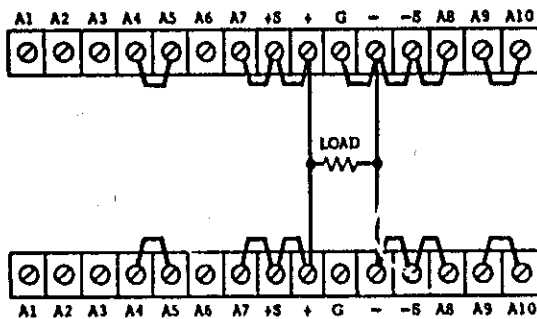
Figure 3-9. Normal Parallel
