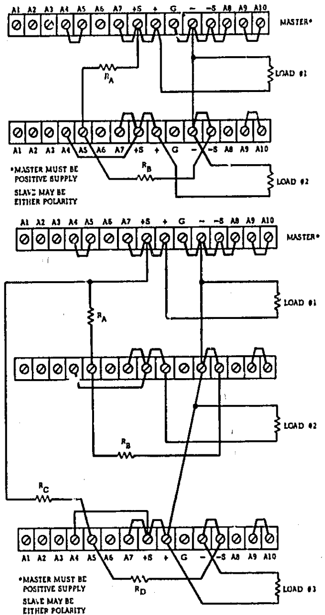
Figure 3-10. Auto-Tracking, Two and Three Units
