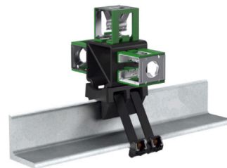
Snap-in Adapter with Universal Angle Adapter base 900639-10
