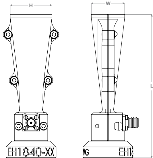
Dimensional drawing
