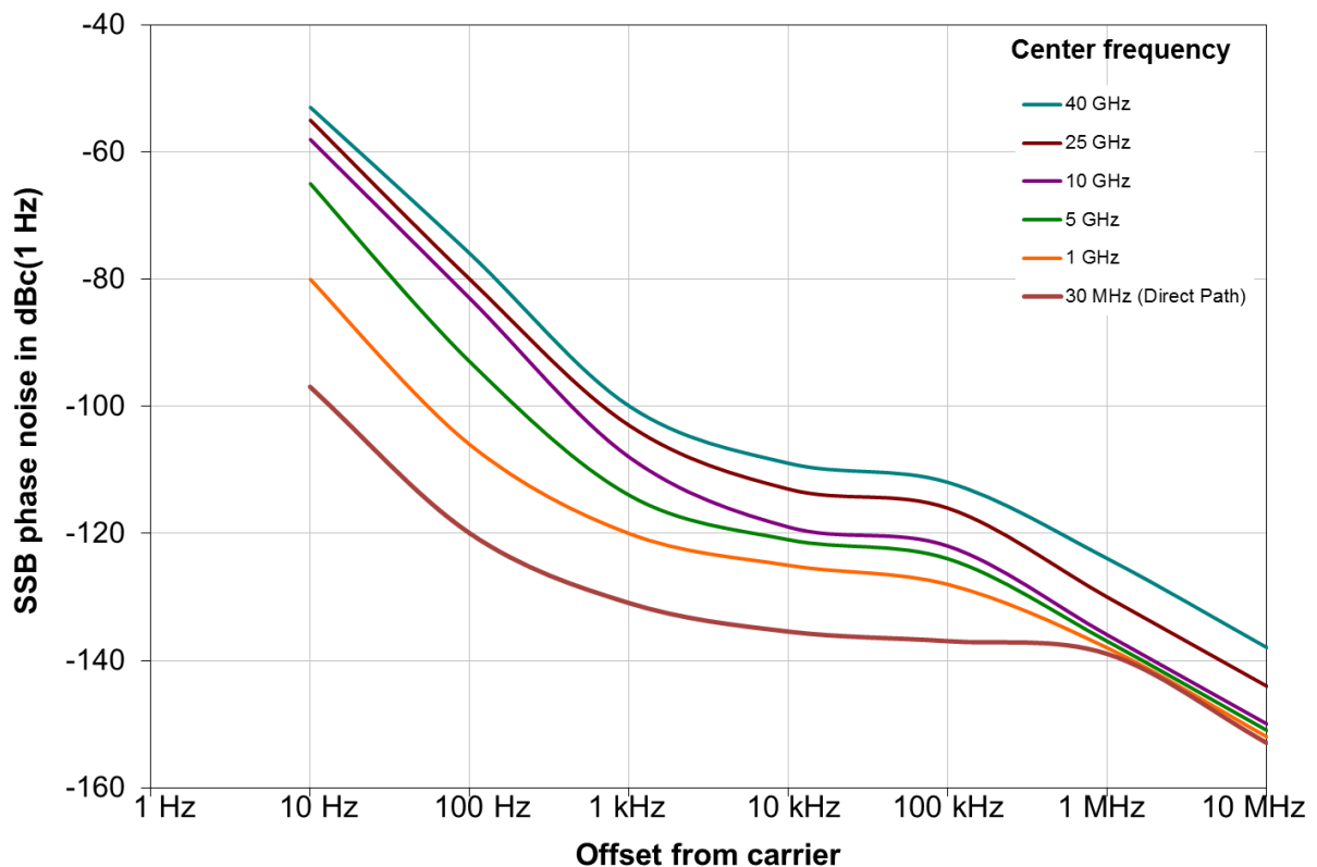
Typical phase noise at different center frequencies (without option R&S®B710)
