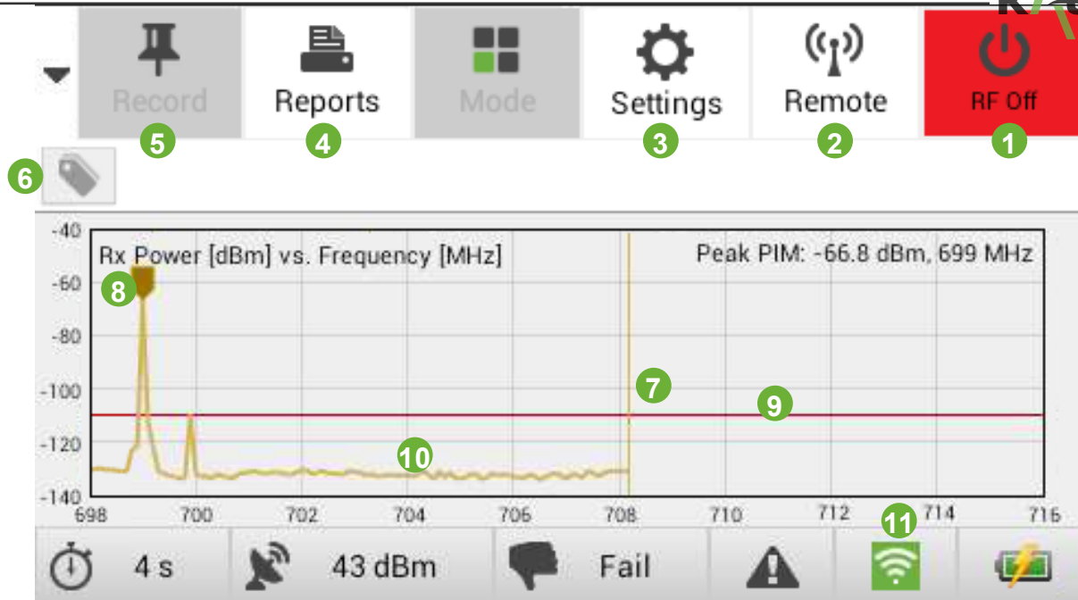
Figure 37 Spectrum Analyzer Measurement Window (Local Display)
