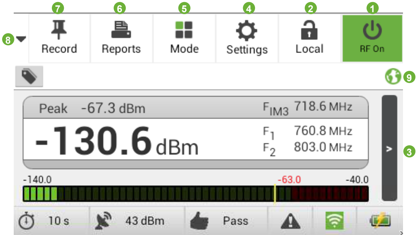
Figure 5 iPA Fixed Frequency Window (Default Measurement Mode)
