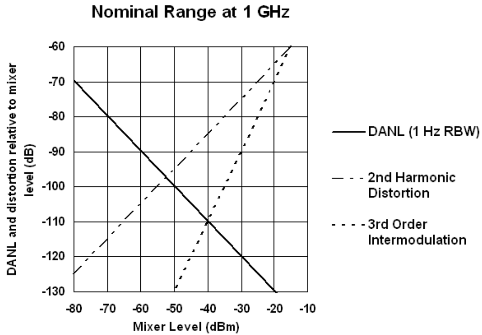
Nominal Dynamic Range Bands 1-4 for Freq Option ≤ 526 [Plot]
