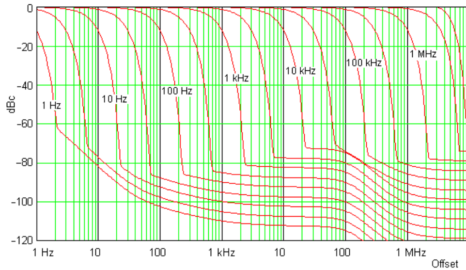
Nominal Dynamic Range vs. Offset Frequency vs. RBW for Freq Option ≤ 526 [Plot] (MY/SG/US5648>SN prefix ≥MY/SG/US5340, ship standard with N9010A-EP3, SN prefix ≥MY/SG/US5648, ship standard with N9010A-EP5)
