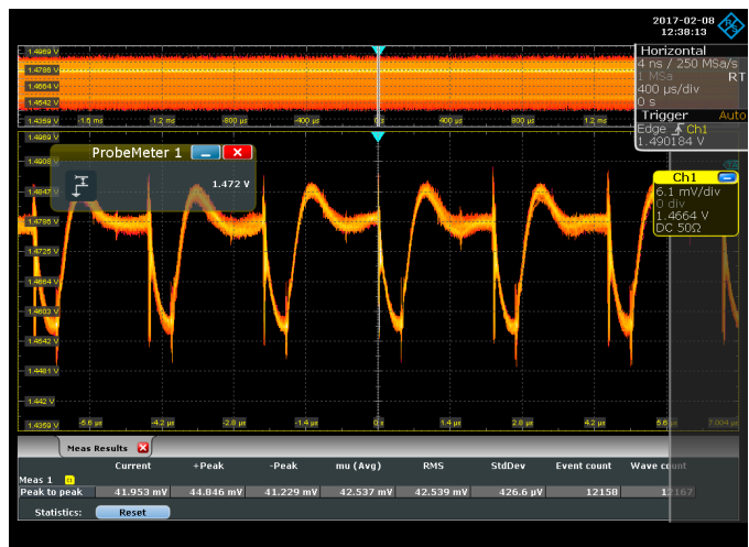
Accurately verify DC level and power supply load response during initialization of a DDR memory with the R&S®RT-ZPR power rail probe and its integrated high-precision R&S®ProbeMeter
