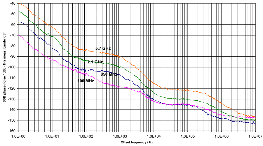
Measured SSB phase noise, unmodulated
