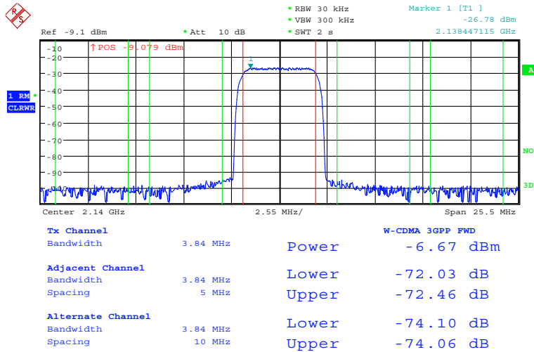
Measured ACPR for 3GPP test model 1, 64 DPCH (baseband gain: +3 dB).
