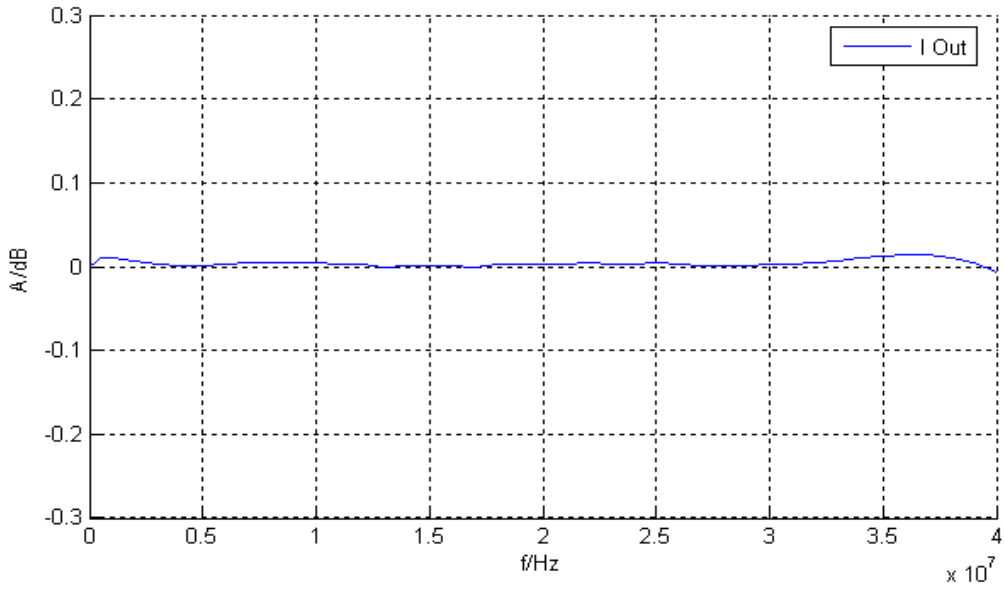
Measured frequency response of I/Q outputs.
