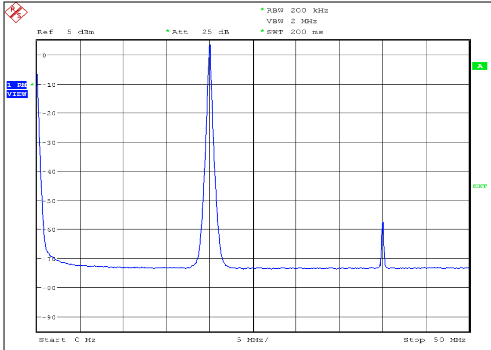
Measured SFDR of I/Q outputs.
