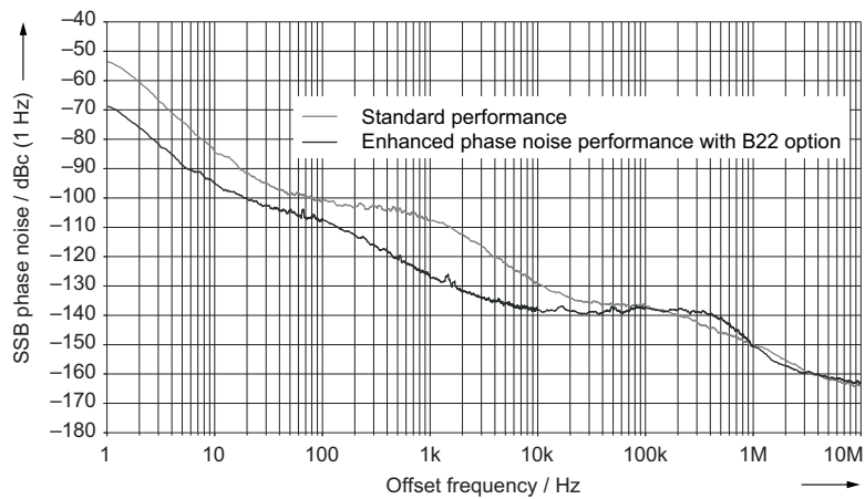
Measured SSB phase noise, f = 1 GHz, comparison of standard performance and performance with R&S ® SMU-B22 option.
