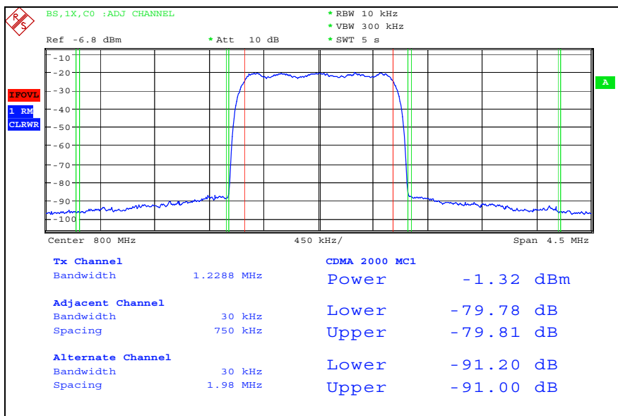
Measured ACPR for a CDMA2000® 1x signal consisting of F-PICH, F-SYNC and one F-FCH.
