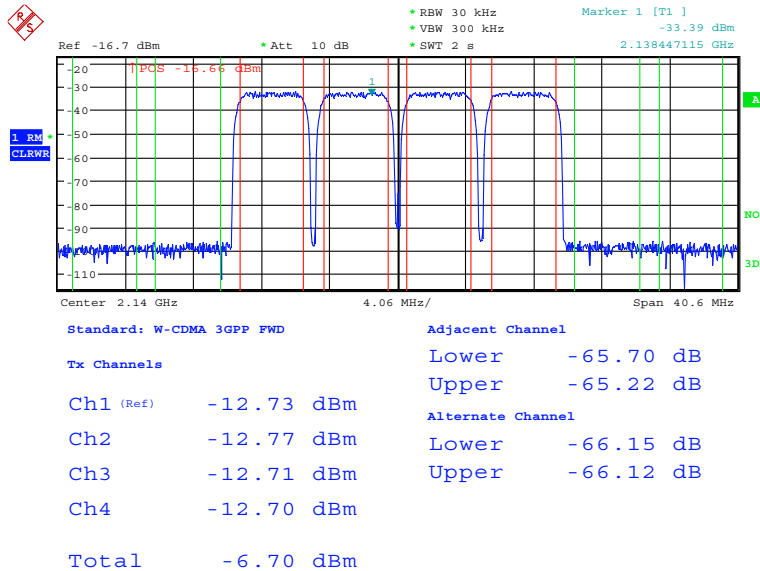
Measured ACPR for a 3GPP four-carrier signal with test model 1, 64 DPCH on each carrier (baseband gain: +3 dB).
