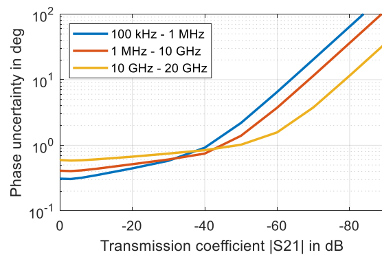
Typical uncertainty of transmission magnitude and transmission phase measurements for the R&S®ZNB20 in the frequency range from 100 kHz to 20 GHz; Analysis conditions: S_{11} = S_{22} = 0 , cal. power –10 dBm, meas. power –10 dBm
