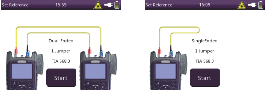
Fig. 11 One jumper reference: single-mode remote and single-mode loopback
