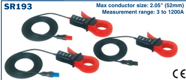
Set of three color-coded SR193 (1200A) current probes Catalog #2140.10 (10 ft leads); Catalog # 2124.25 (30 ft leads)
