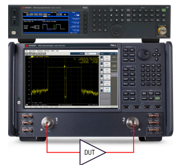
Classic NPR measurement with PNA-L and UXR
