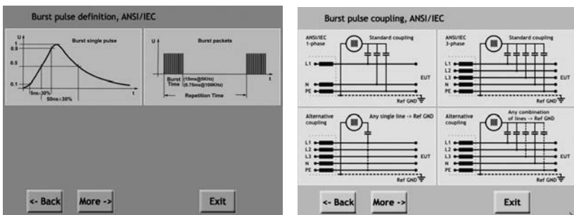
Example burst pulse graphs
