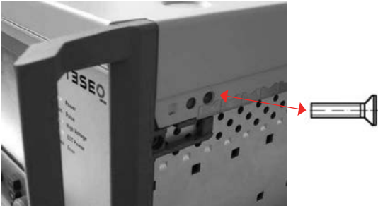
Removing the NSG 3040 side panels and cover
