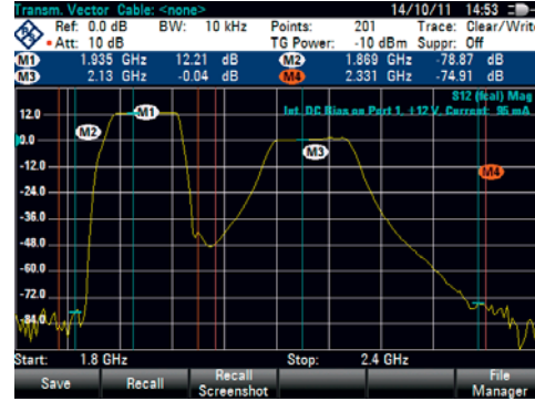
Two-port capability for transmission measurements.
